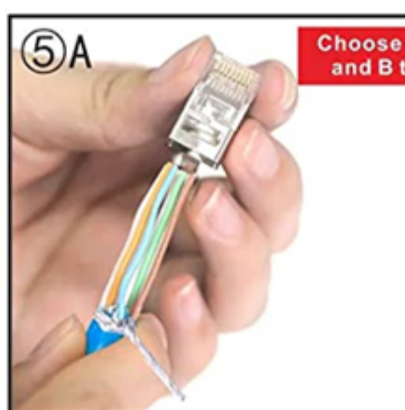
⑤A: Insert the wires into the RJ45 connector
