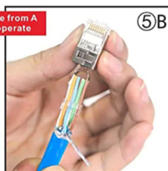
⑤B: Thread the wires through the load bar, assemble plug
