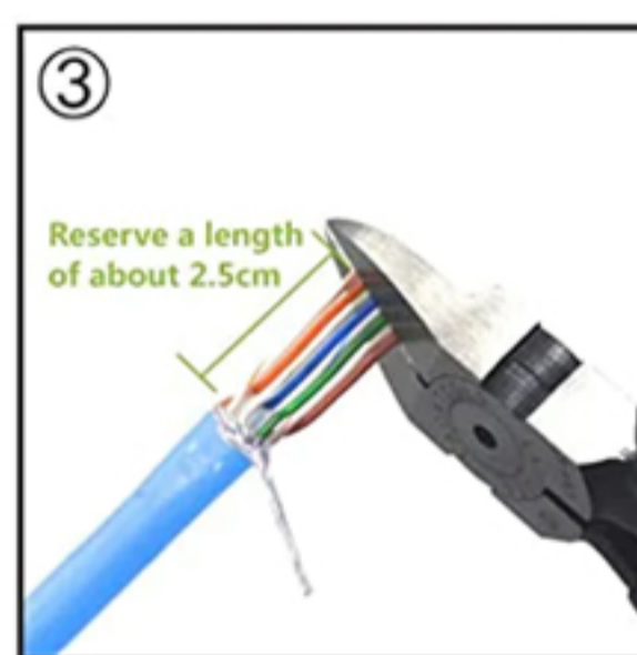
③ Cut the wires to 2.5cm long
