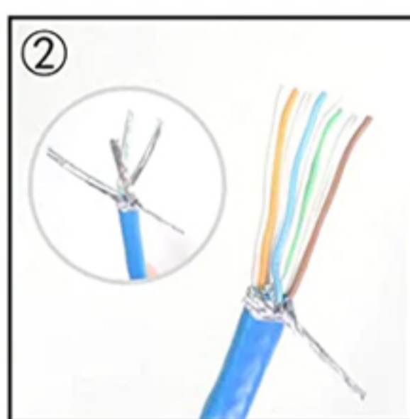
② Cut the extra braid, aluminum foil and PET off
