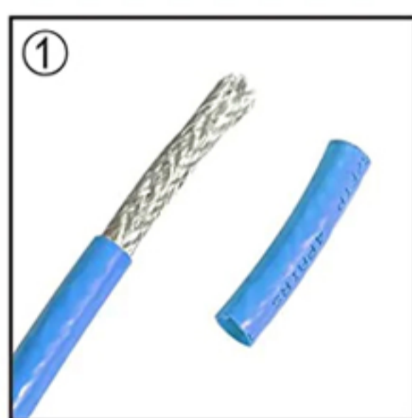
① Strip the cable jacket about 3cm
